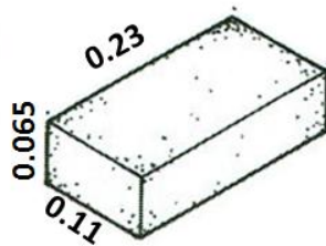
Ladrillo tayuyo 0.065x0.11x0.23
