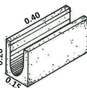
Block "U" 0.15x0.20x0.40
