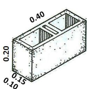
Block 0.15x0.20x0.40
